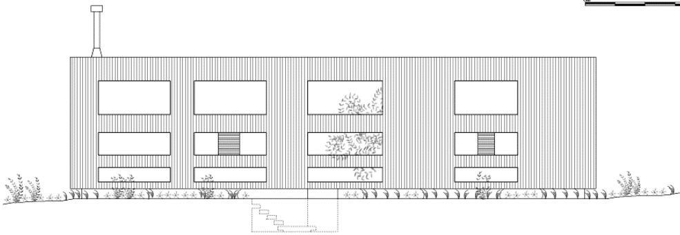
East Elevation
