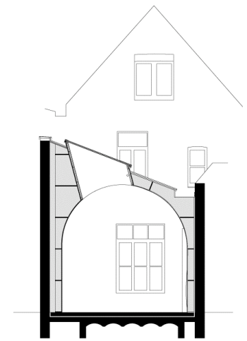
sections C-C scale 1/100
