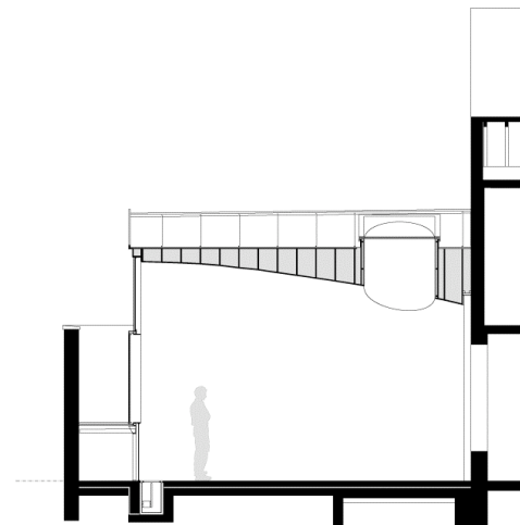
sections A-A scale 1/100
