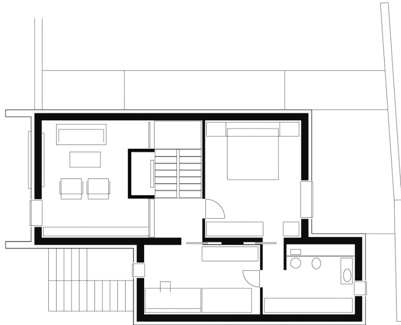
first floor, main house
