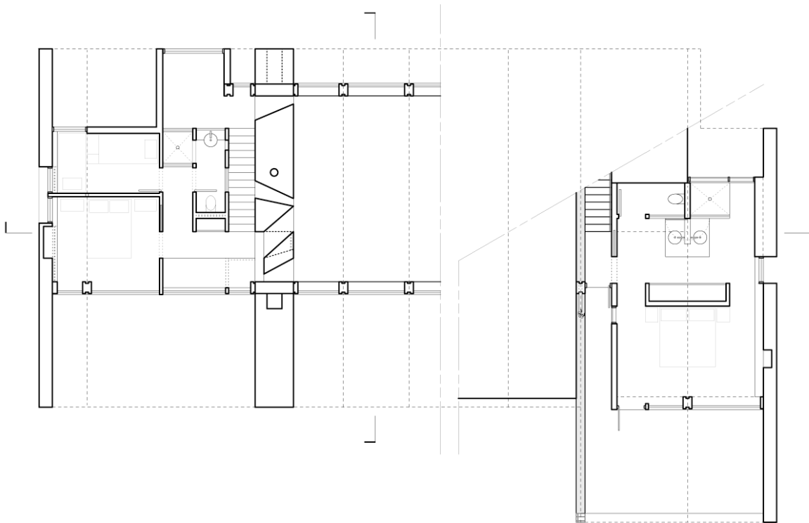
UPPER / LOWER FLOOR PLANS 0 5' 10'
