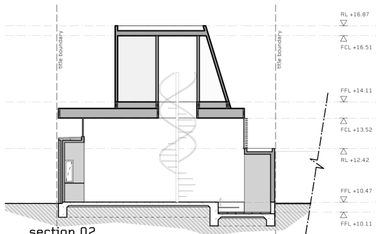
section 02
