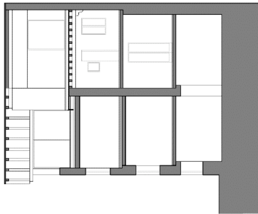
CROSS SECTION - LOUNGE
