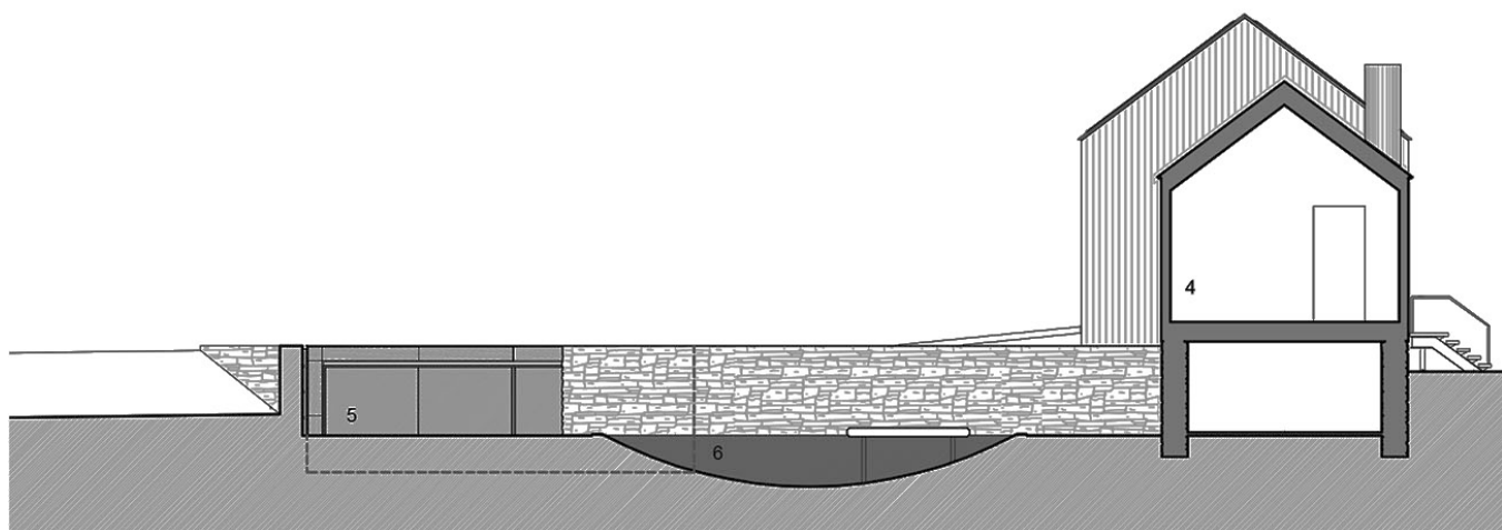
section west - east
