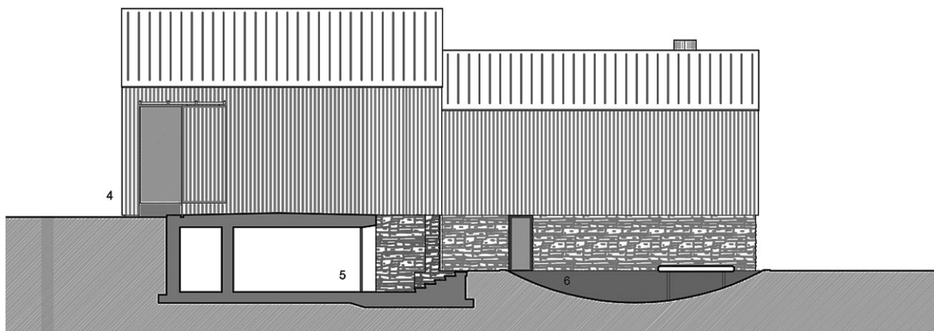
section north - south
