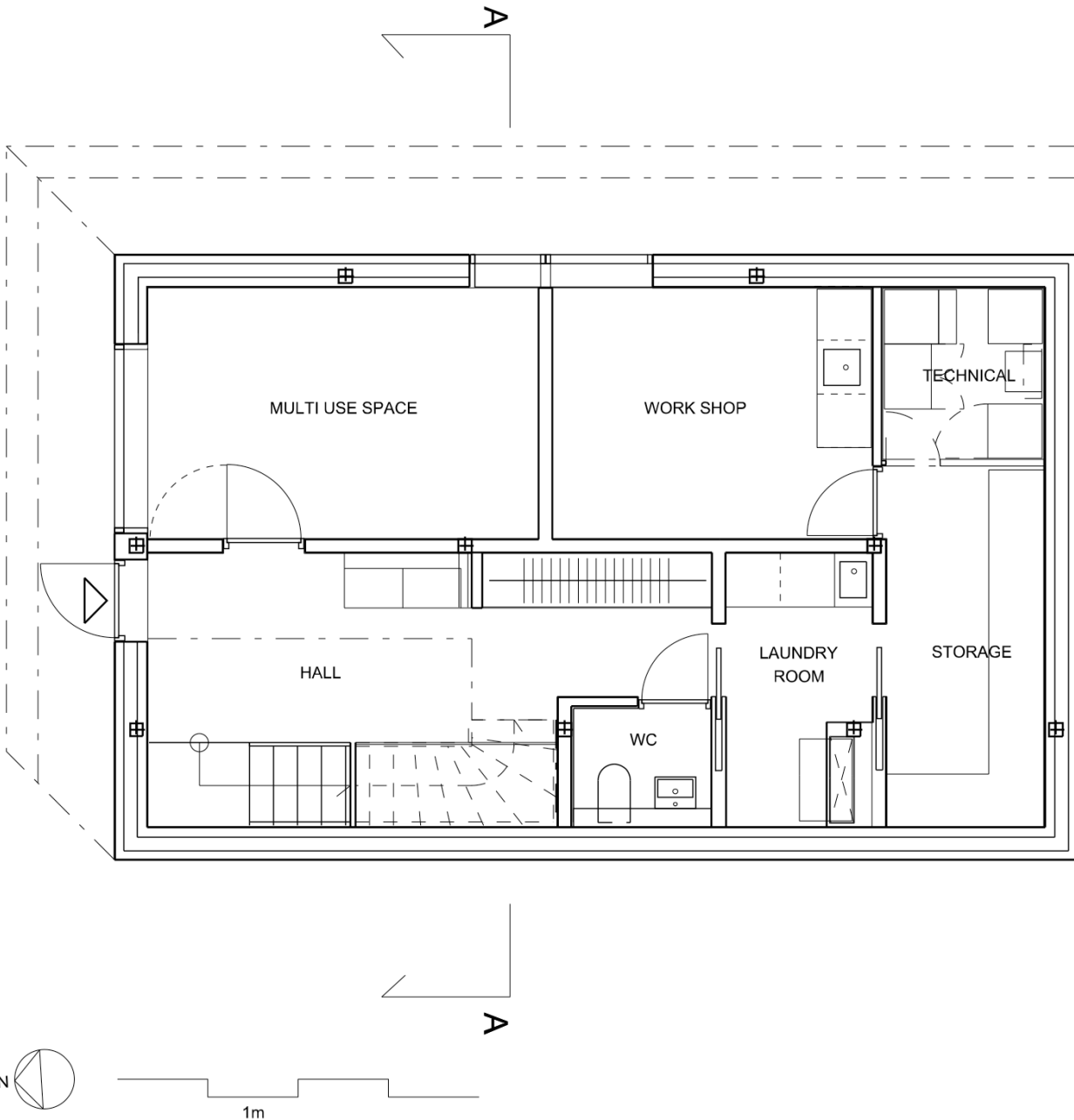
PLAN -1
