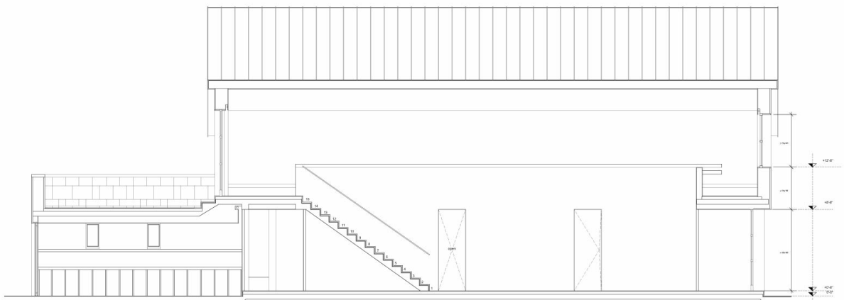
02 Section B-B. Scale 1:1/4"
