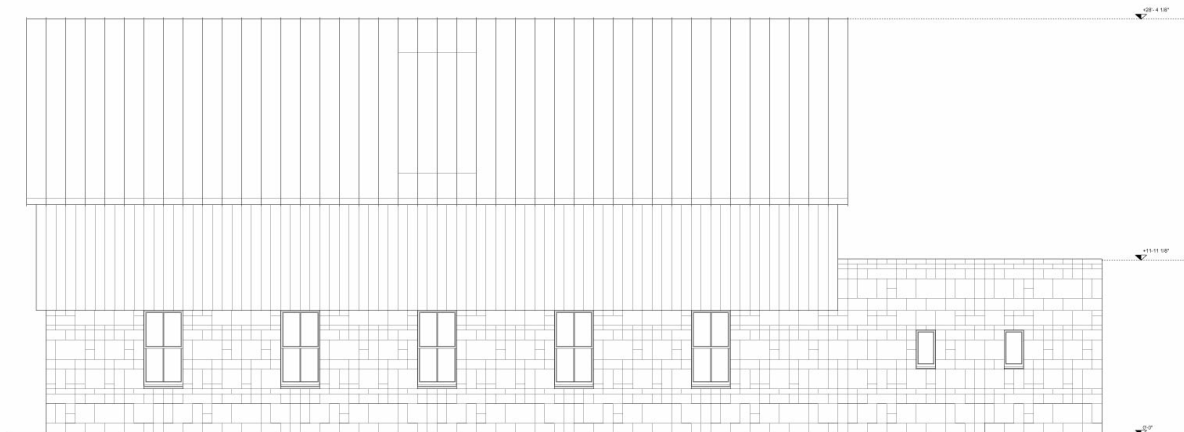
01 Alder Street elevation. Scale 1:1/4"
