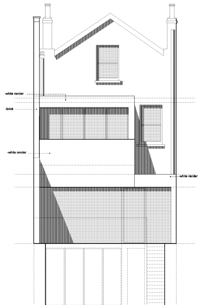
REAR ELEVATION
