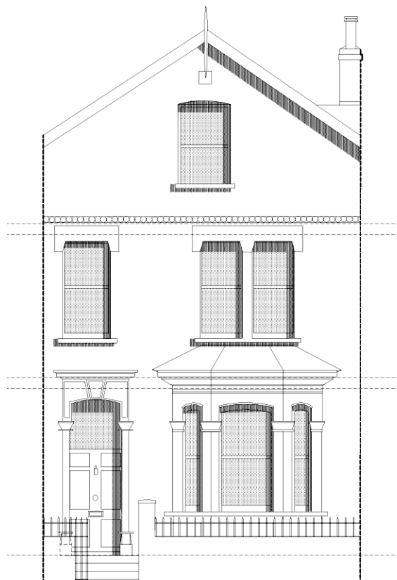
FRONT ELEVATION
