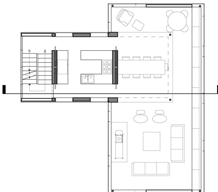
FOURTH FLOOR PLAN
